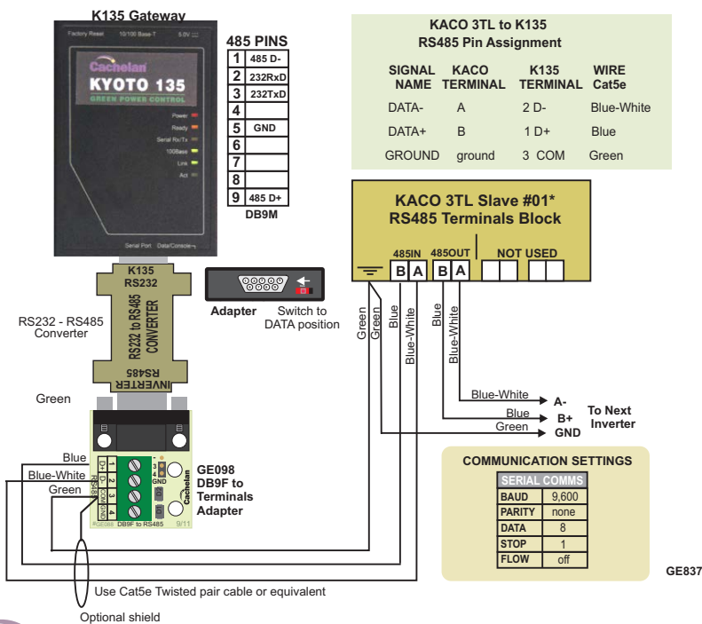
Fig 2 K135-KACO XP10U RS485 connections
